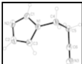
Fig. 1. Molecular structure of 3-(1 H -imidazol-1-yl)propanenitrile with atom labelling scheme. Displacement ellipsoids are drawn at the 50% probability level.
